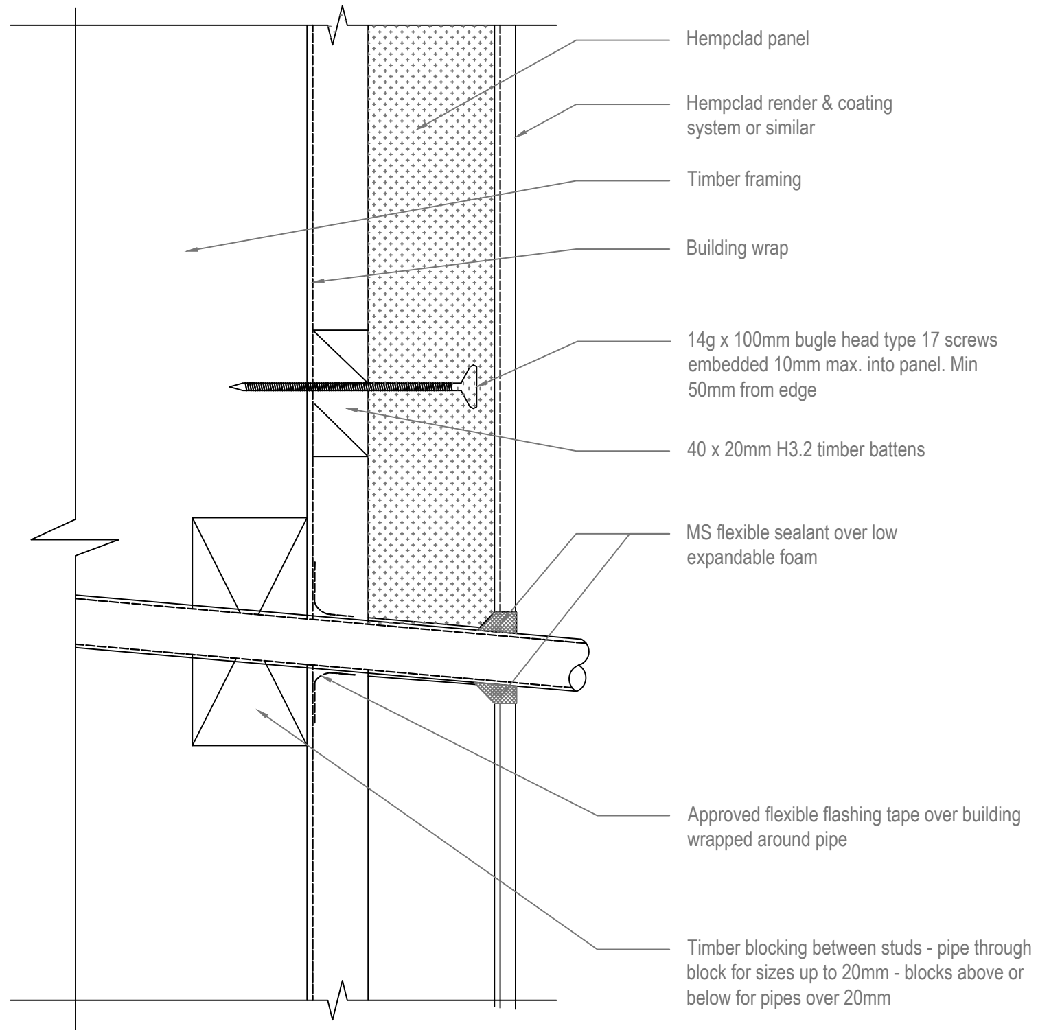
PIPE PENETRATION DETAIL 07
