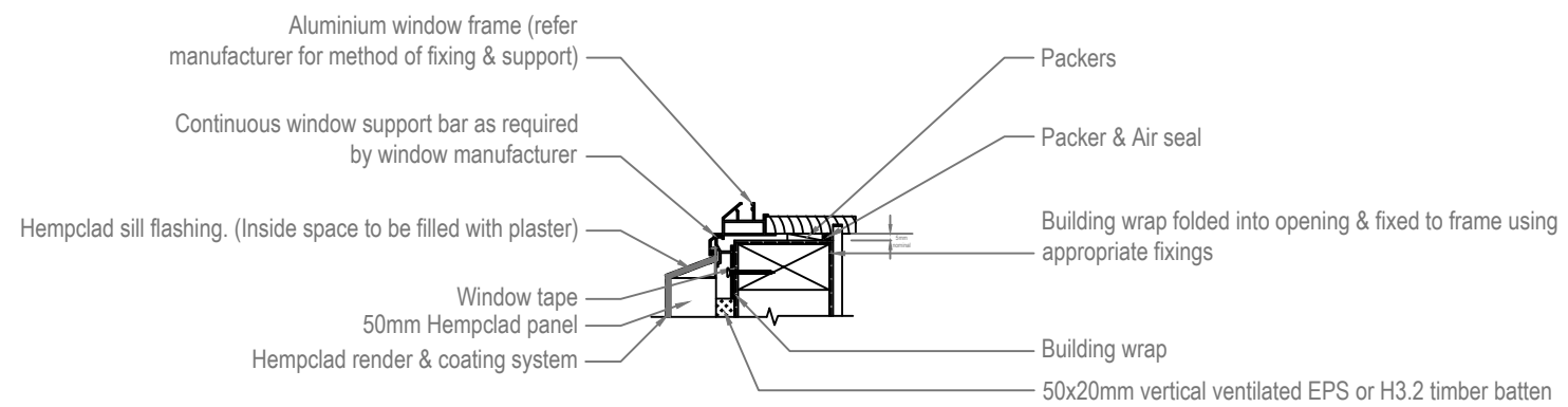
OPENING FLASHINGS - WINDOW SILL DETAIL 05
