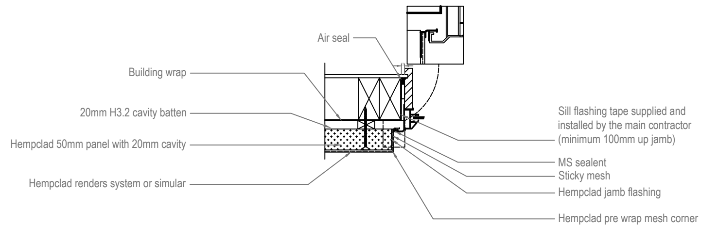
OPENING WINDOW JAMB FLASHING DETAIL 04
