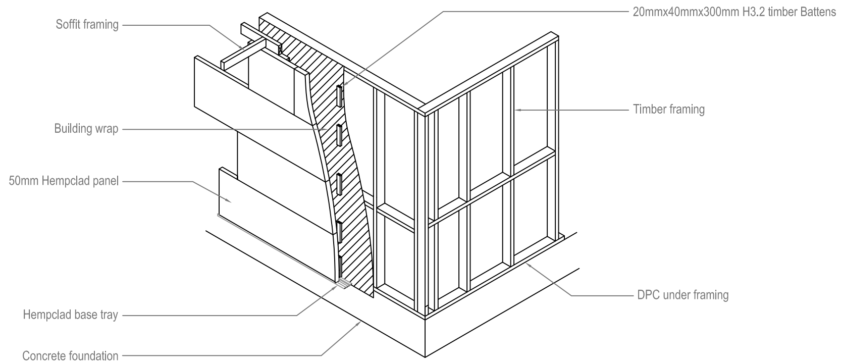
BATTEN AND PANEL LAYOUT CONCRETE FLOOR WITHOUT REBATE DETAIL 01
