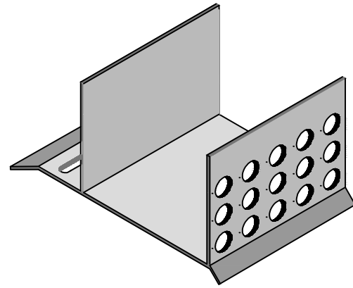
50mm Panel base tray / Cavity for Hempclad 50mm panel
