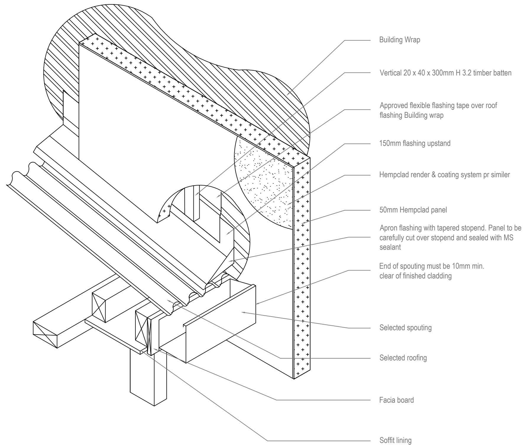
ROOF / WALL JUCTION - KICKOUT FLASHING DETAIL 13
