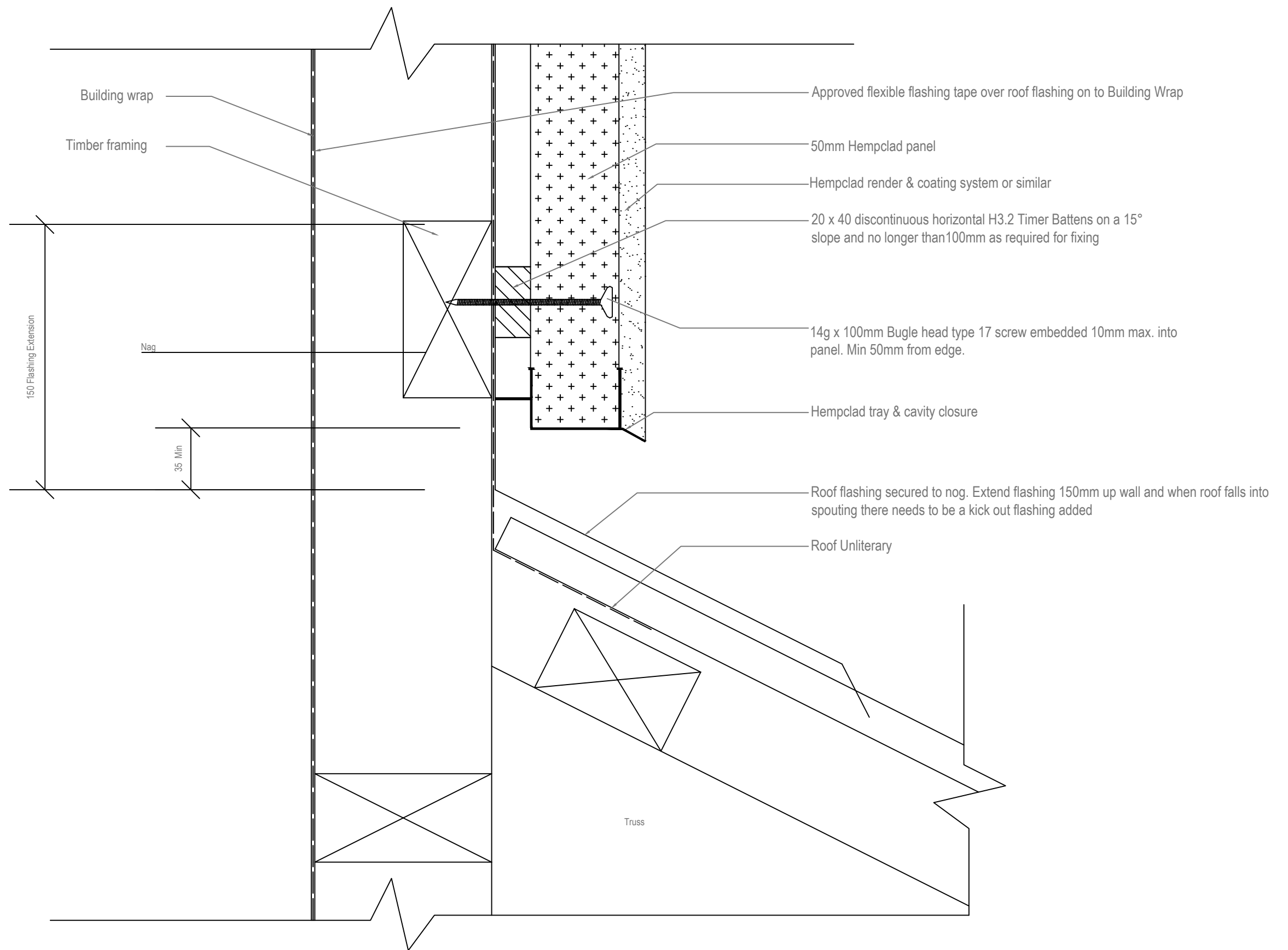
ROOF / WALL JUNCTION DETAIL 12
