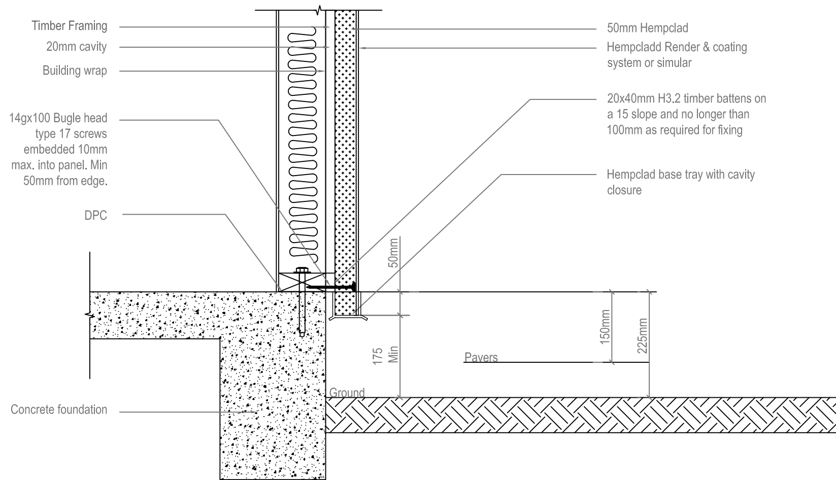
CONCRETE FOUNDATION DETAIL 02
