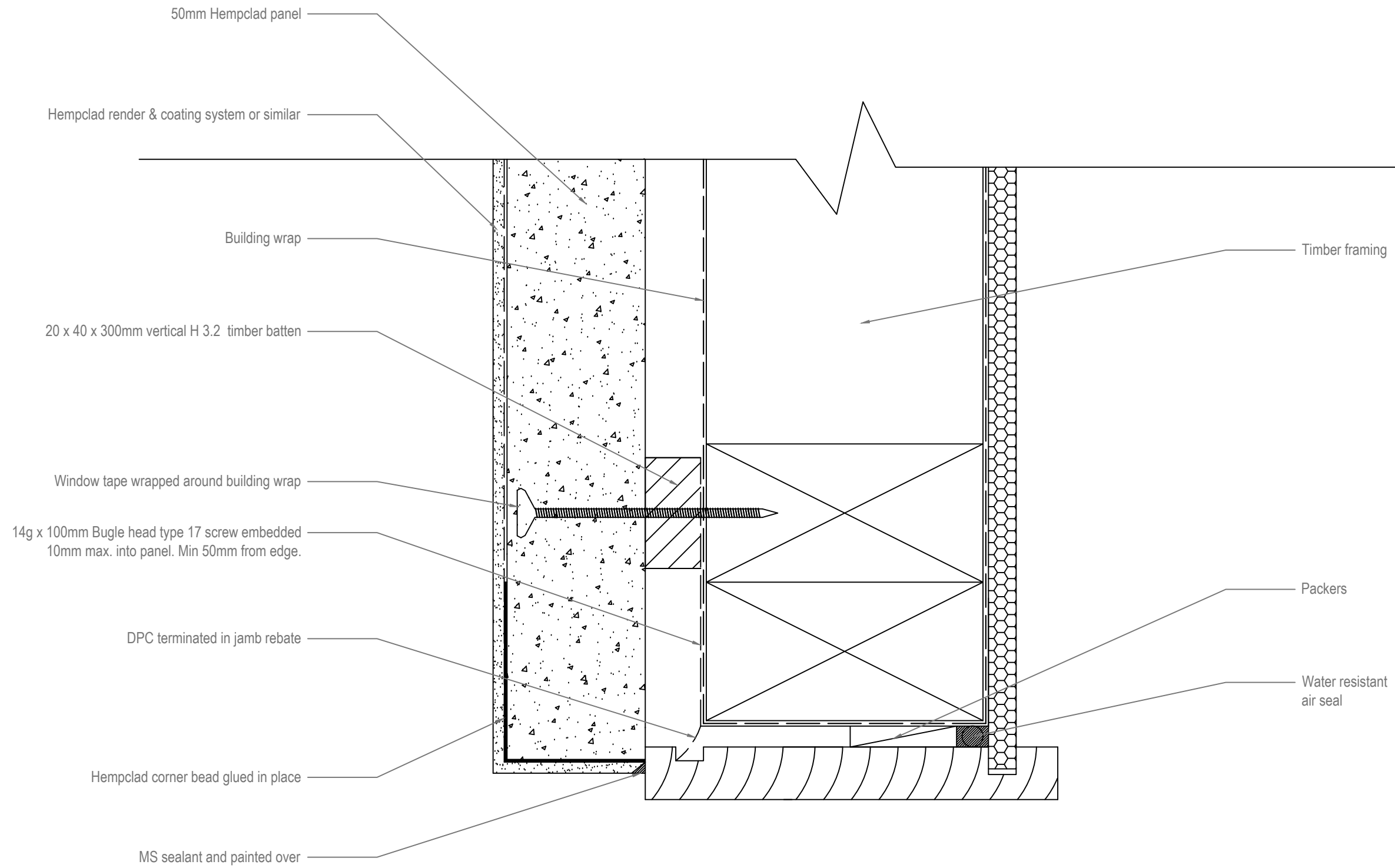
OPENING FLASHING GARAGE DOOR - Jamb DETAIL 9
